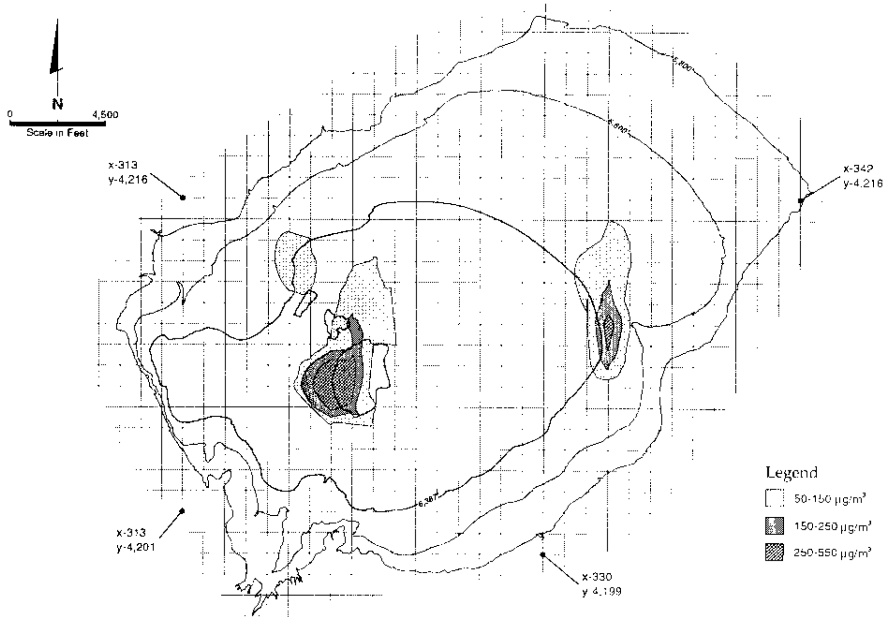
Figure 3II-30. FDM Modeling Results for a Lake Elevation of 6,387 Feet on the Maximum Episode Day
