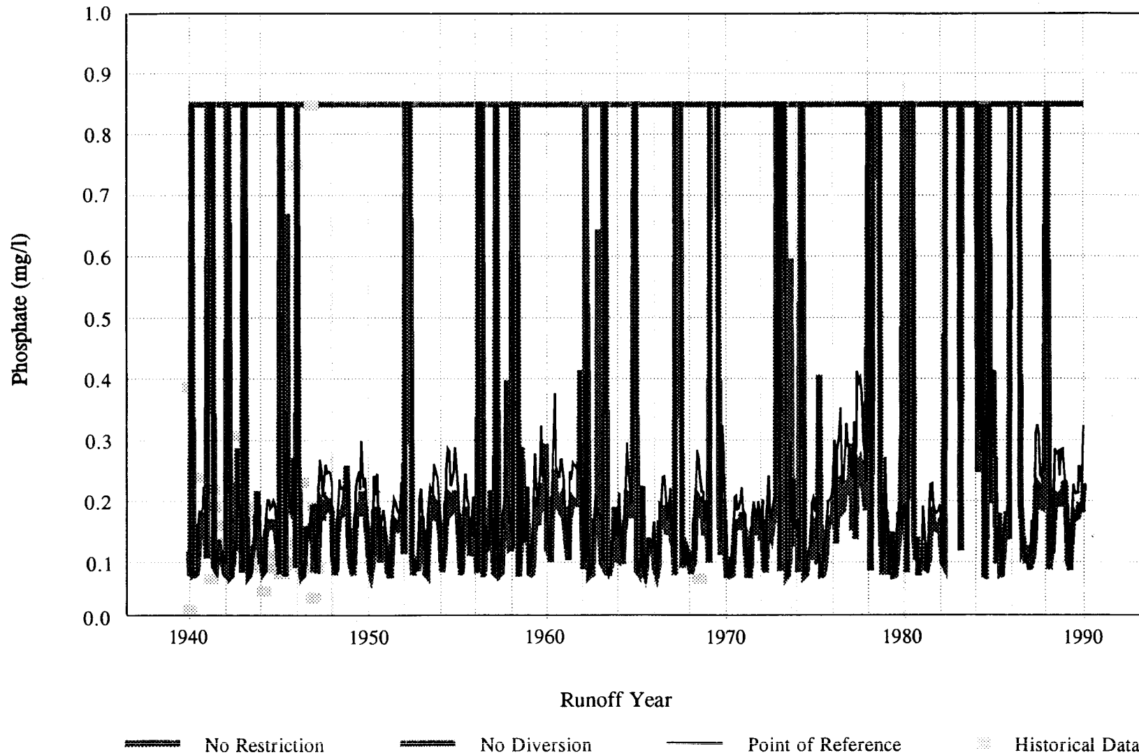
Figure 3B-14. Predicted and Historical Phosphate Concentrations for East Portal Outflow from 1940 to 1990
