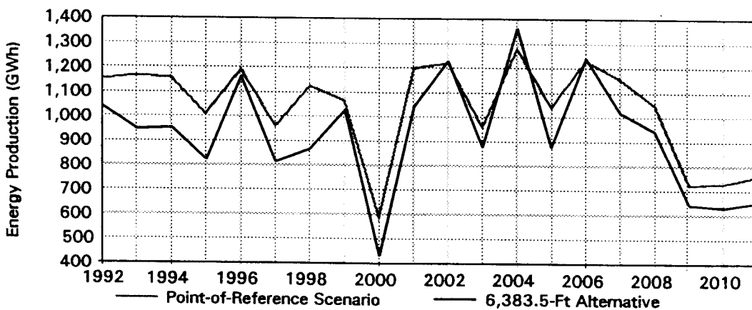
Figure 3M-8a. Energy Production for the No-Restriction, 6,372-Ft, 6,377-Ft, and 6,383.5-Ft Alternatives Compared to the Point-of-Reference Scenario
