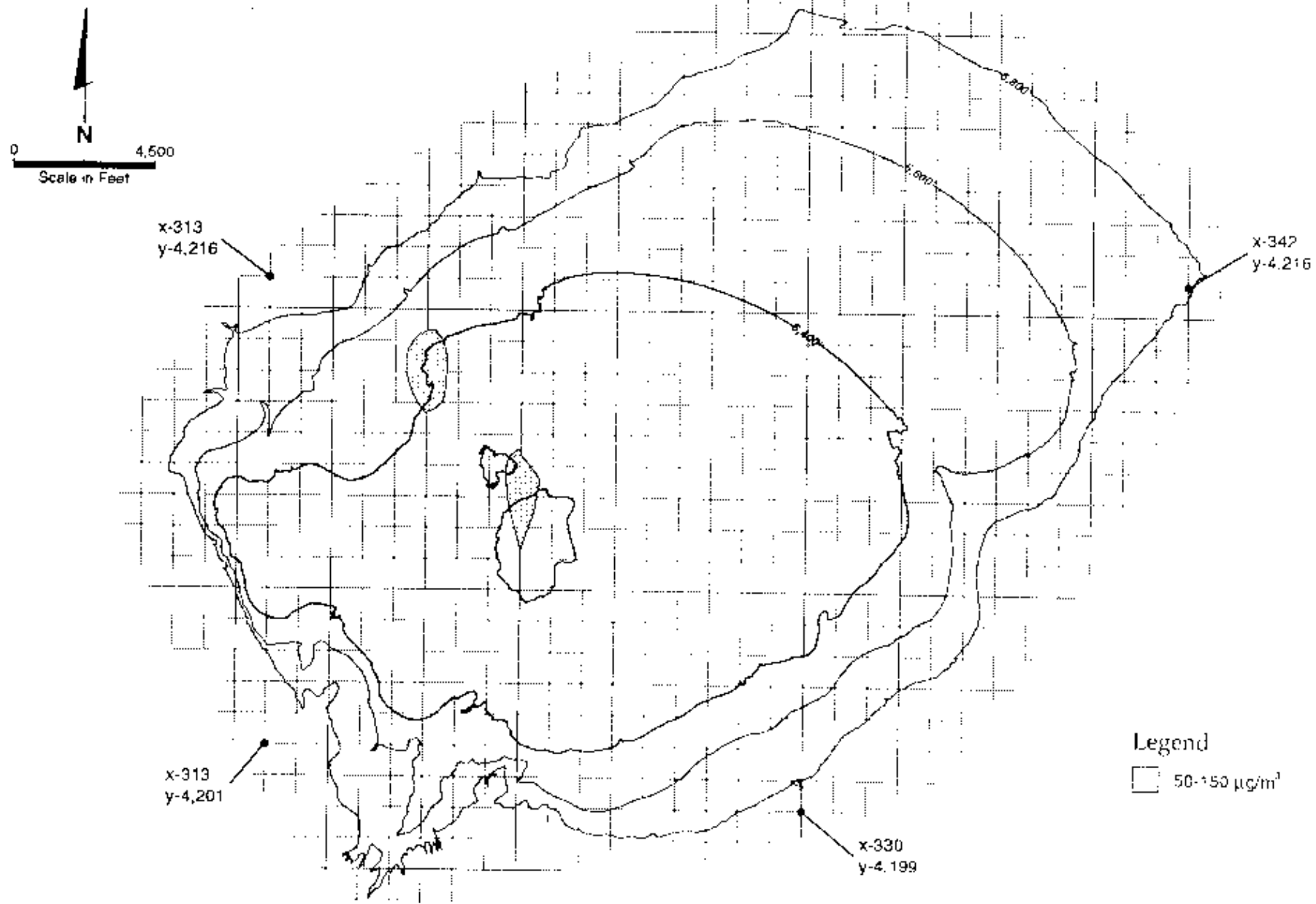
Figure 3H-32. FDM Modeling Results for a Lake Elevation of 6,400 Feet on the Maximum Episode Day
