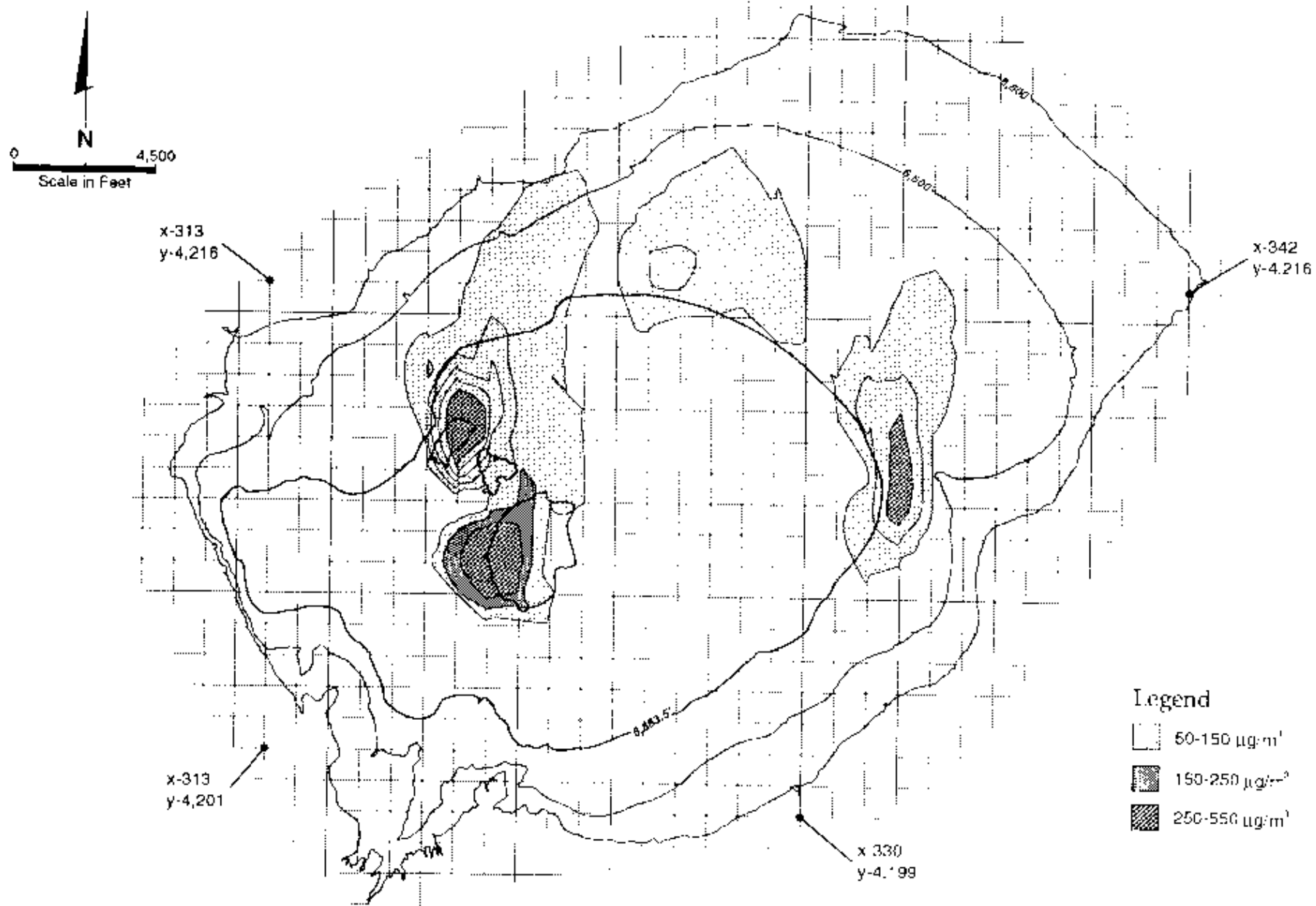
Figure 3H-29. FDM Modeling Results for a Lake Elevation of 6,883.5 Feet on the Maximum Episode Day
