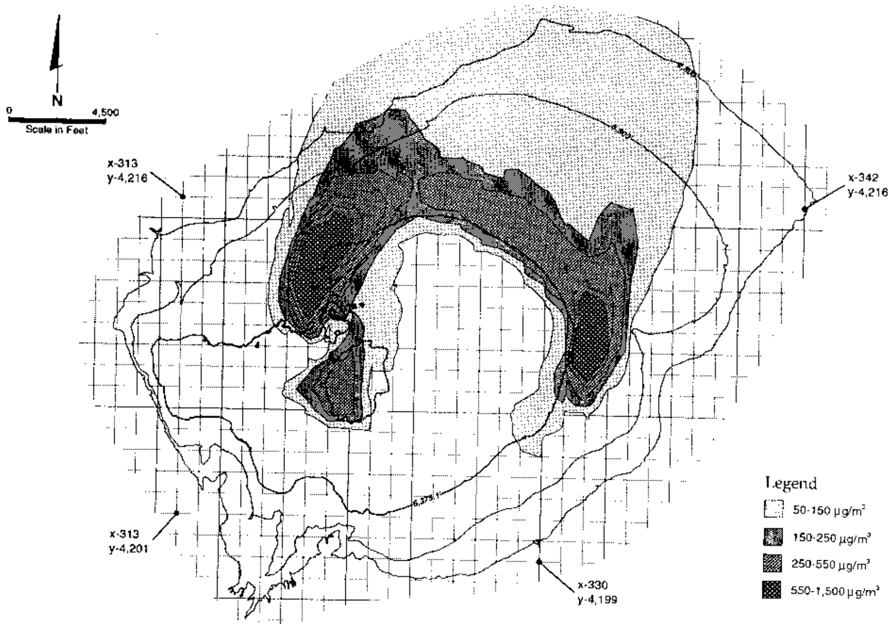
Figure 3H-25. FDM Modeling Results for a Lake Elevation of 6,375.1 Feet on the Maximum Episode Day
