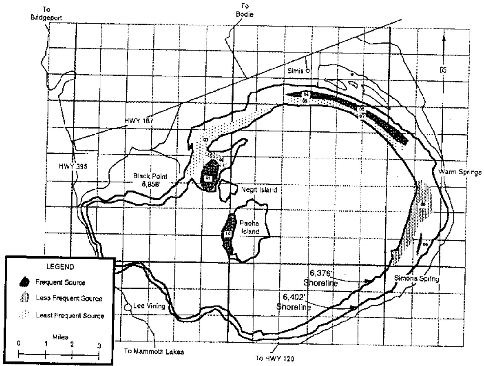
Figure 3H-18. Approximate Source Areas during Dust Storms Observed by GBUAPCD
