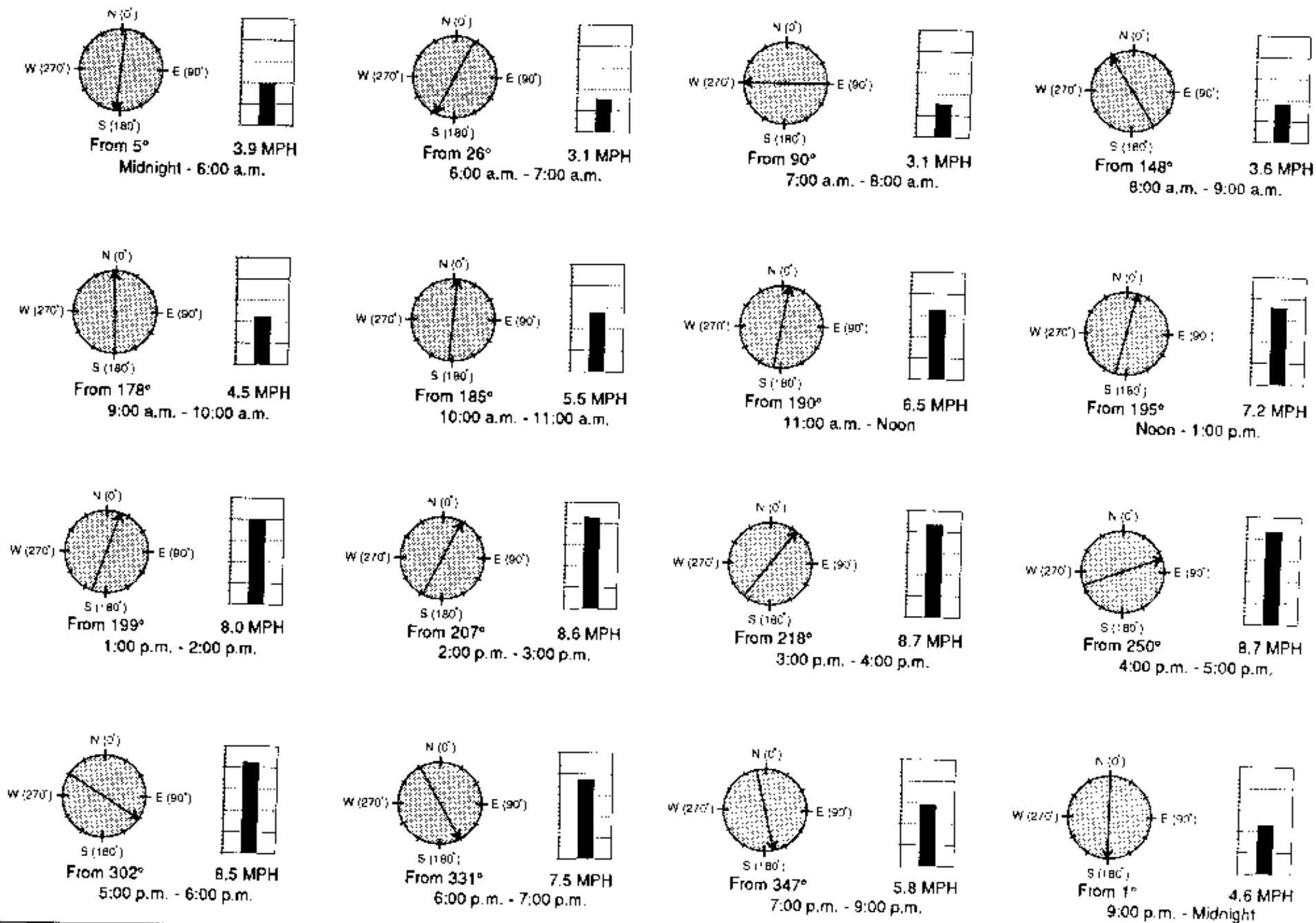
Figure 3H-6. Average Time-of-Day Wind Patterns for the Simis Ranch Monitoring Site, 1986-1991
