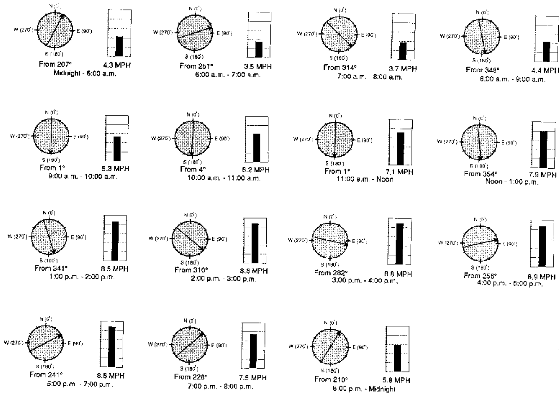
Figure 3H-5. Average Time-of-Day Wind Patterns for the Lee Vining Monitoring Site, 1986-1991
