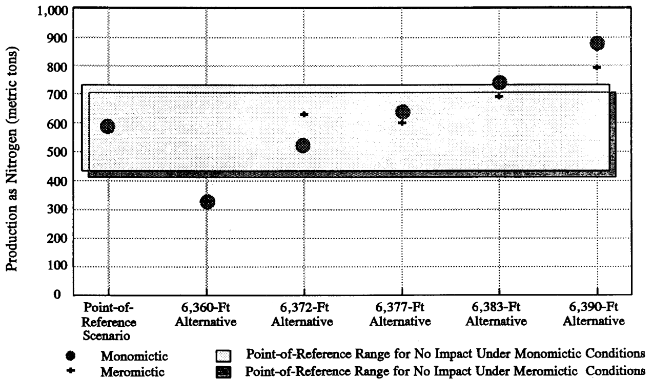
Figure 3E-21b. Predicted Brine Shrimp Production Lakewide Totals
