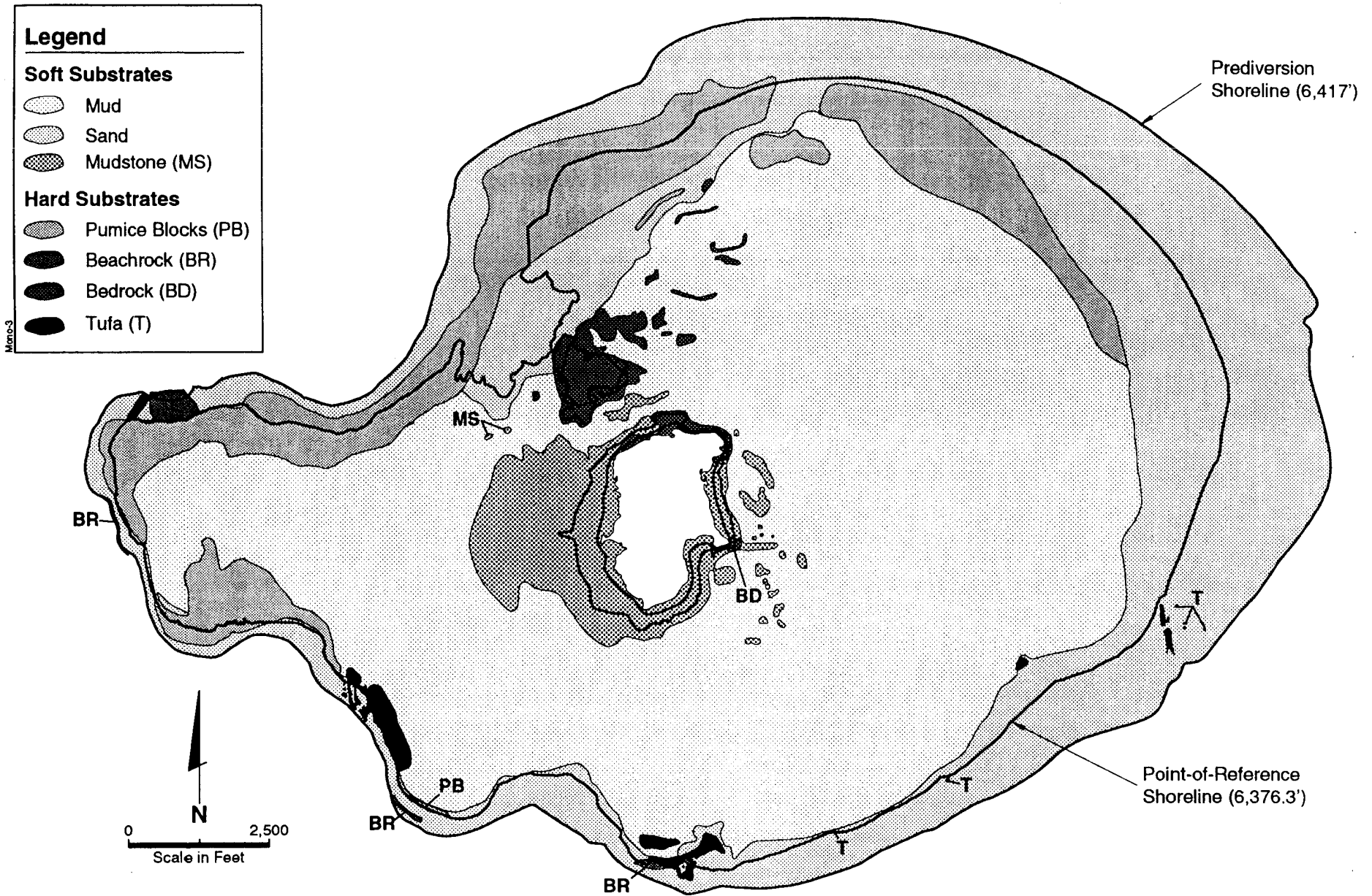
Figure 3E-8. Substrates at Mono Lake
