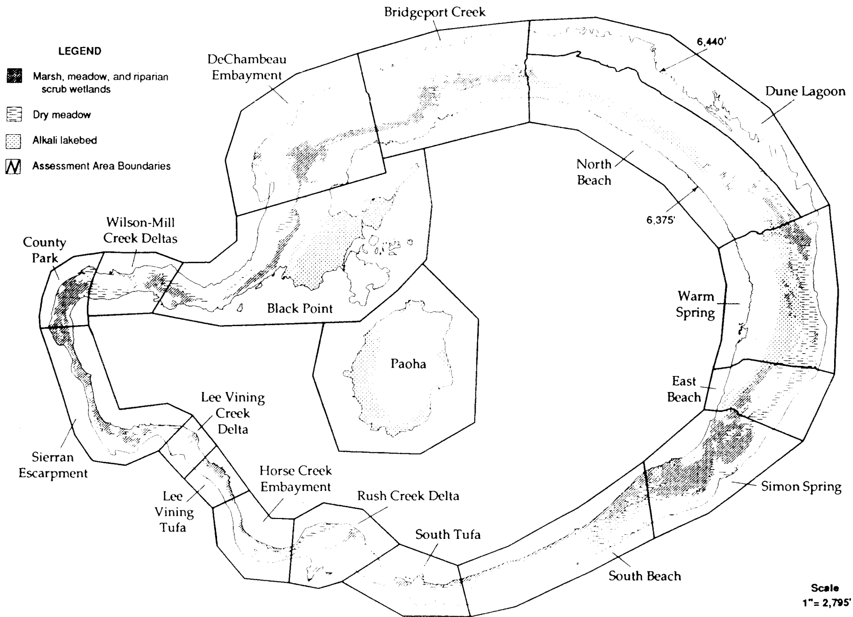
Figure 3C-10. Lake-Fringing Wetlands under Point-of-Reference Conditions
