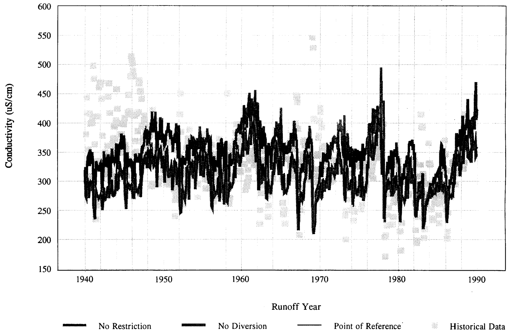
Figure 3B-8. Predicted and Historical Conductivity for LA Aqueduct Filtration Plant Inflow from 1940 to 1990
