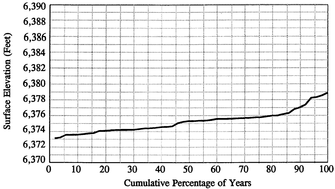
Figure 3A-14. Simulated Mono Lake Surface Elevation 6,372-Ft Alternative
