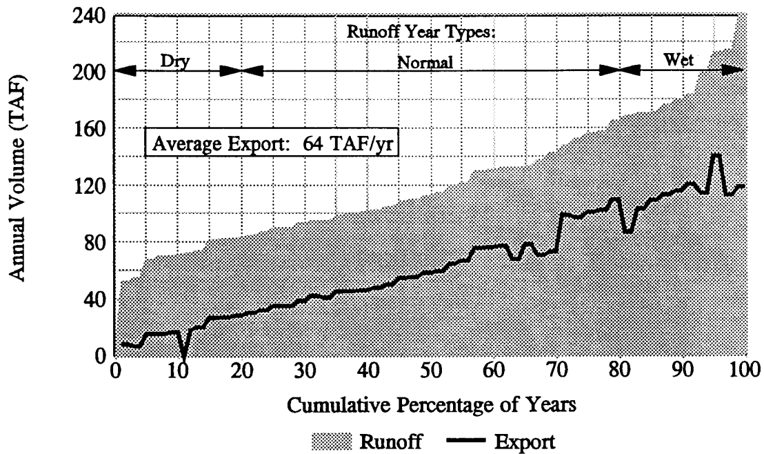
Figure 3A-15. Frequency Distribution of Runoff and Simulated Mono Basin Exports 6,372-Ft Alternative
