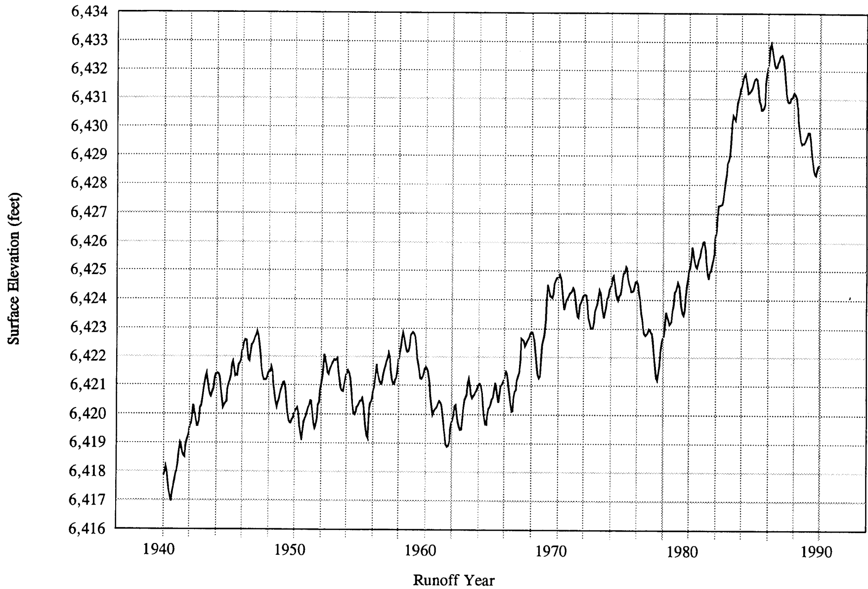
Figure 3A-8. Simulated Mono Lake Surface Elevation in the Absence of LADWP Diversions, 1940-1989
