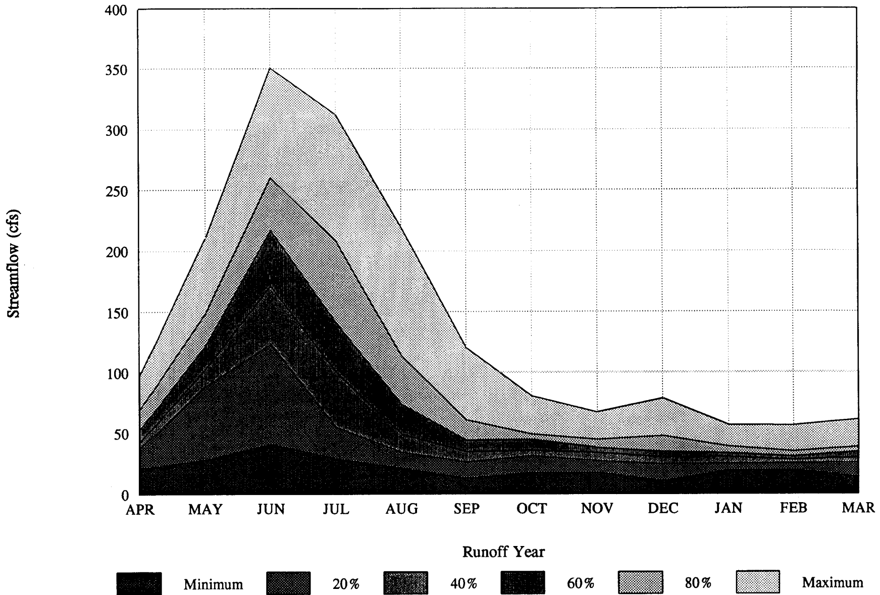
Figure 3A-2. Monthly Lee Vining Creek Streamflow Distribution
