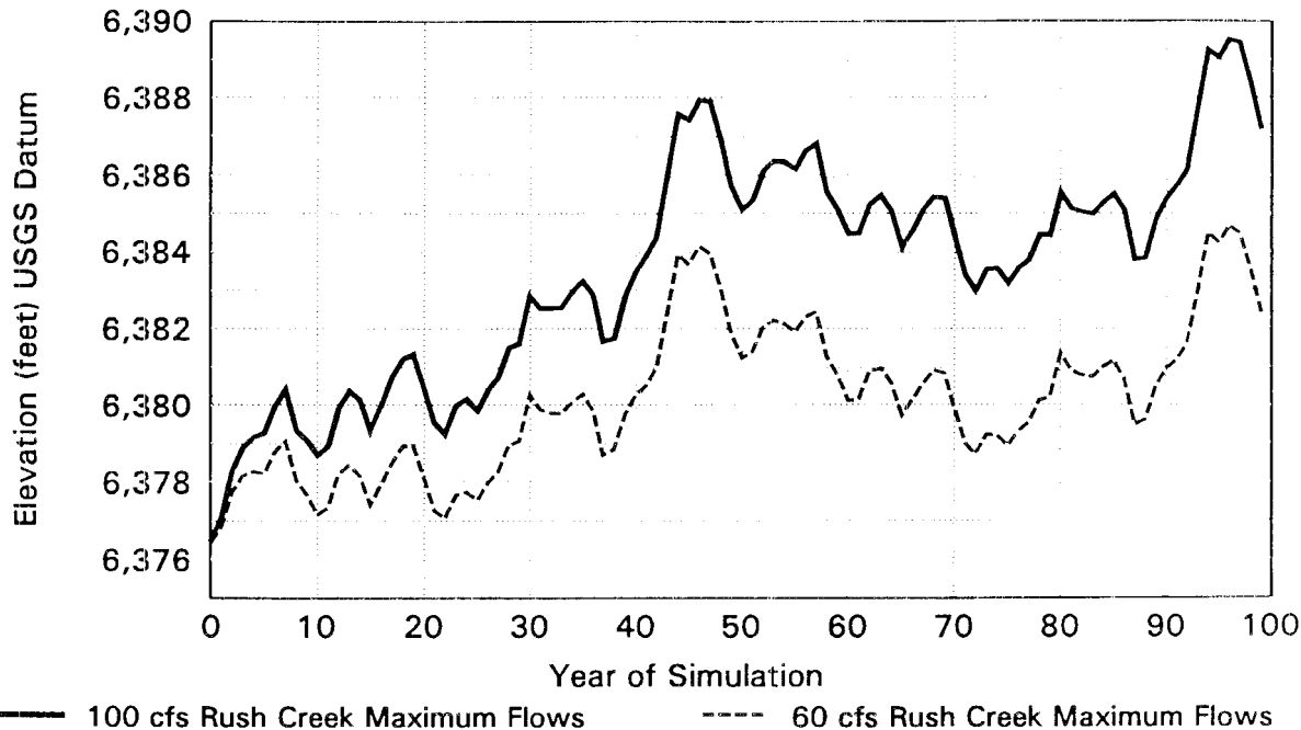
Figure 2-17. Simulated Lake Surface Elevation with Preliminary Minimum Monthly Streamflows from DFG Stream Evaluation Reports
