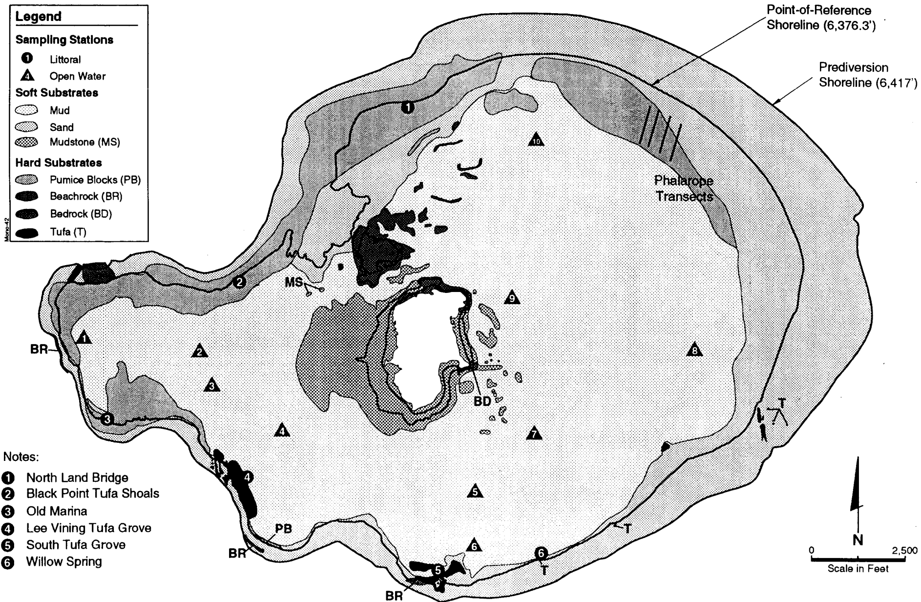
Figure 3E-17. Substrates at Mono Lake and 1991 Littoral and Open Water Sampling for Alkali Flies
